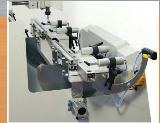
Trave a 0°
